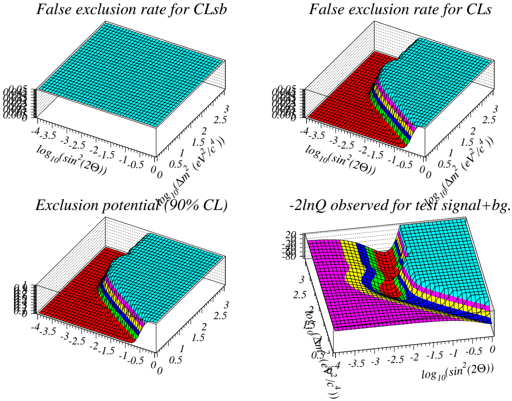
Fig. 3: A study of a toy neutrino oscillations experiments. Upper left: The false exclusion rate (for 95% CL) for CL_{s+b} . Upper right: The false exclusion rate (for 95% CL) for CL_s . Lower left: The exclusion potential for CL_s (for 90% CL). Lower right: The observed -2 \ln(Q) for the test signal experiment (the upper right corner is cut off at z = -2 \ln(Q) = 20 but rises sharply to very high values).
