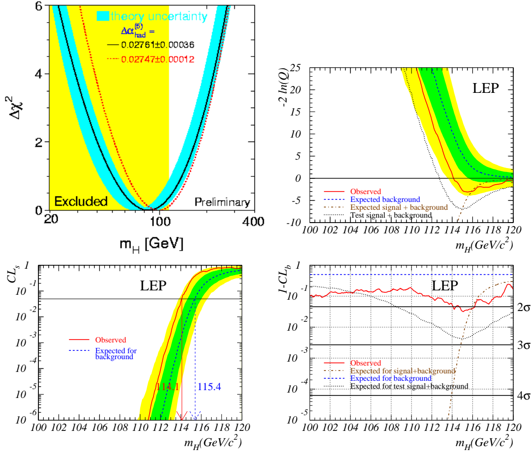
Fig. 2: Preliminary results from the combined Higgs search at LEP. Upper left: Indirect evidence for the Higgs from the global electroweak fit. Upper right: Minus twice the log-likelihood ratio versus m_H for the direct search. Lower left: The approximate signal confidence CL_s(m_H) and the derived exclusion interval. Lower right: The test of the signal significance via 1 - CL_b(m_H) .
