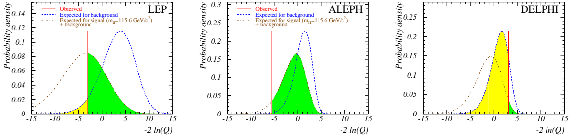
Fig. 5: Preliminary results from the combined Higgs search at LEP. The p.d.f.'s of -2 \ln(Q) for the background hypothesis (p.d.f. on right) and for the background plus a 115.6 \text{ GeV}/c^2 Higgs (p.d.f. on left) together with the observed results.
