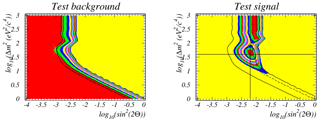
Fig. 4: A study of a toy neutrino oscillations experiments. Left: The exclusion contour for a typical background experiment is close to the expected result (the solid lines). The grey contours show -2 \ln(Q) with the lower left region being close to 0 and the right upper region having very large values (very background-like). The excluded regions are in the upper right. Right: A typical signal+background experiment with \Delta(m^2) = 40 \text{ (eV}/c^2)^2 and \sin^2(2\theta) = 0.006 . The grey contours show -2 \ln(Q) but cut off to focus on the region of the global minima. The leftmost solid line is the expected limit from CL_s , the rightmost solid and dashed lines are the 90% and 10% confidence level limits, respectively.
